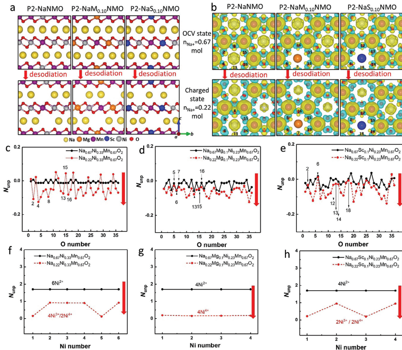
Figure 5. DFT calculations for P2-NaMO, P2-NaM 0.10 NMO, and P2-NaS 0.10 NMO at OCV ( n_{\text{Na}^+} = 0.67 mol) and fully charged state ( n_{\text{Na}^+} = 0.22 mol). a) Atomistic structures by using DFT-PBE+ U . b) Computed spin density plots (an isosurface of 0.006 \text{ eV } \text{\AA}^{-3} ) using DFT-HSE06, the up- and down-spin electrons are in yellow and blue, respectively (The atom colors are the same as in (a), but the isosurfaces distort the colors when overlaid). The number of unpaired electrons N_{\text{unp}} on c–e) O and f,g) Ni for the three materials (black points are for the OCV state and red points are for the fully charged state). The labeled O atoms in (c–e) correspond to the labeled atoms in (b).
